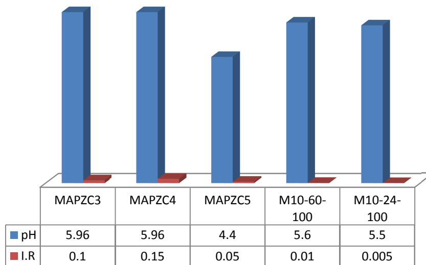
Fig. 4. I.R and pH of the activated carbon of maize cobs
